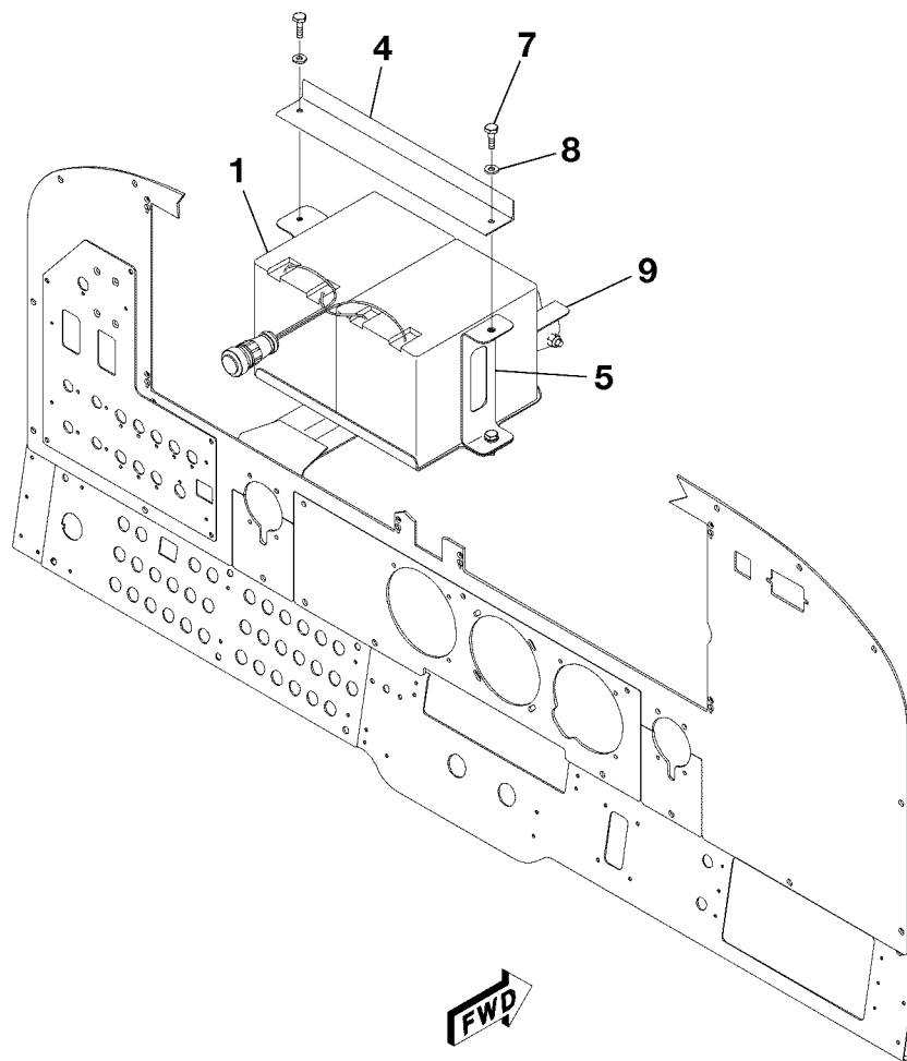
DETAIL A
