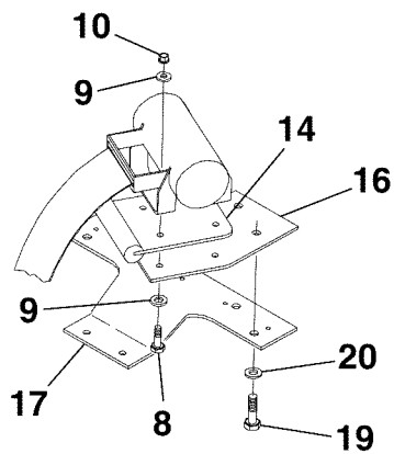
DETAIL C
