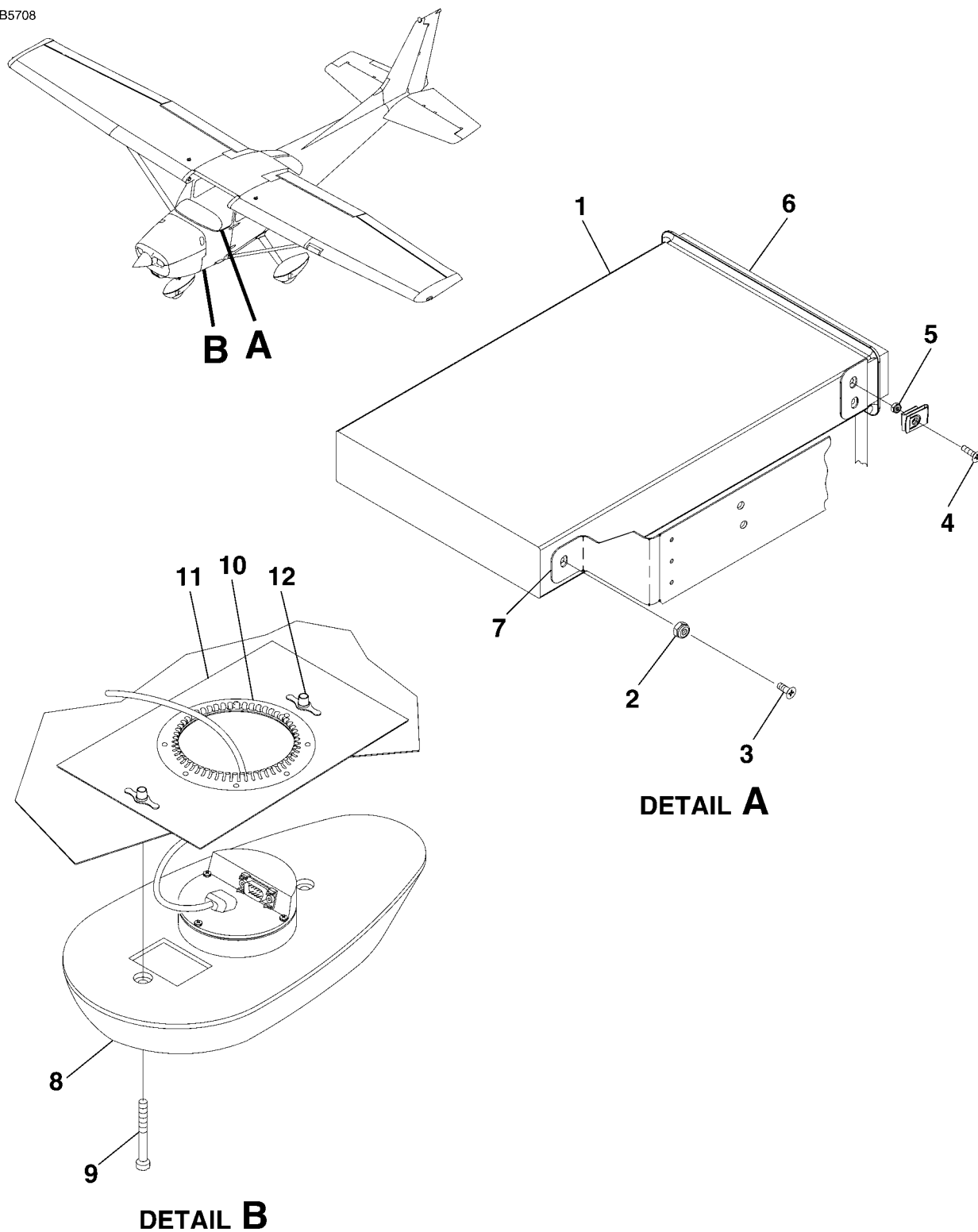
AUTOMATIC DIRECTION FINDING (ADF) NAVIGATION SYSTEM FIGURE 02 (SHEET 1)
