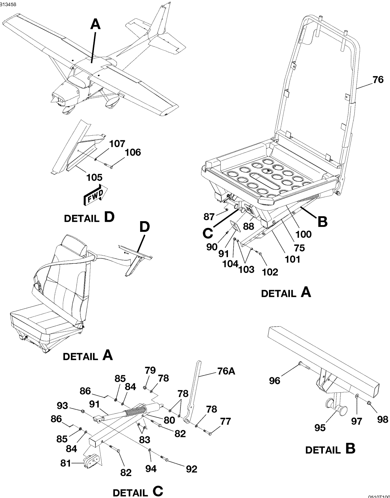
OBSERVER SEAT INSTALLATION - OPTIONAL FIGURE 05 (SHEET 2)
