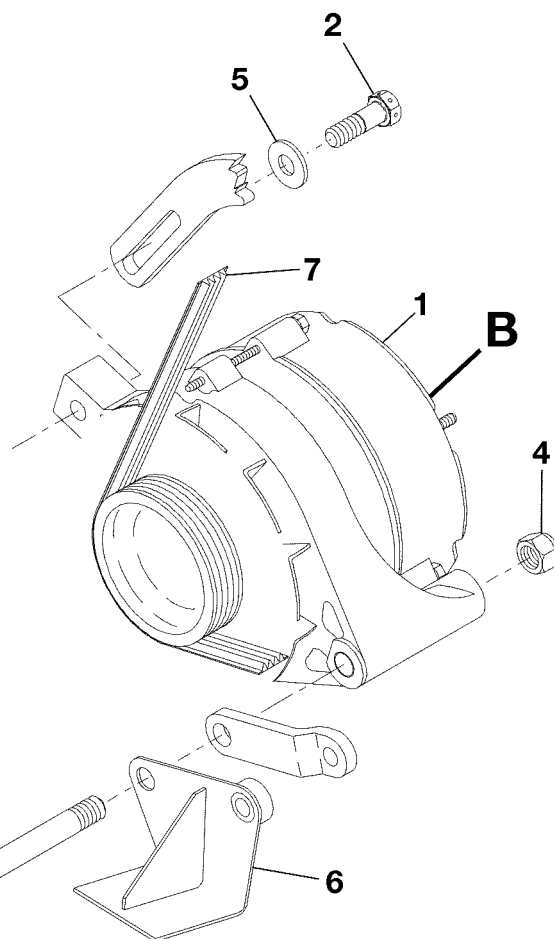
DETAIL A
