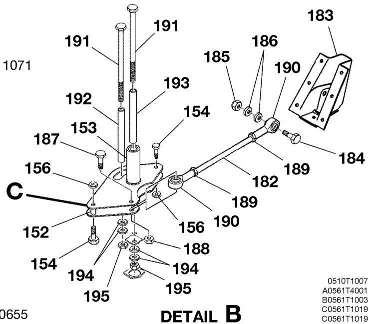
AILERON CONTROL SYSTEM FIGURE 03 (SHEET 3)
