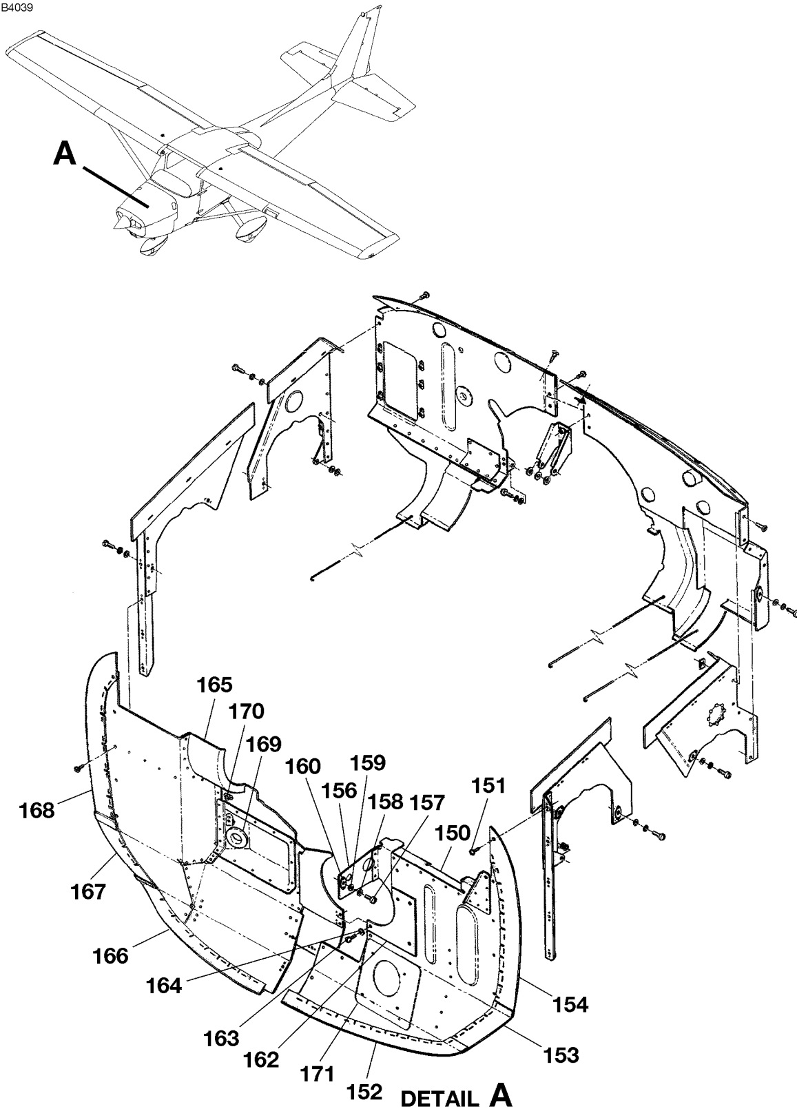
ENGINE BAFFLES INSTALLATION FIGURE 01 (SHEET 3)
