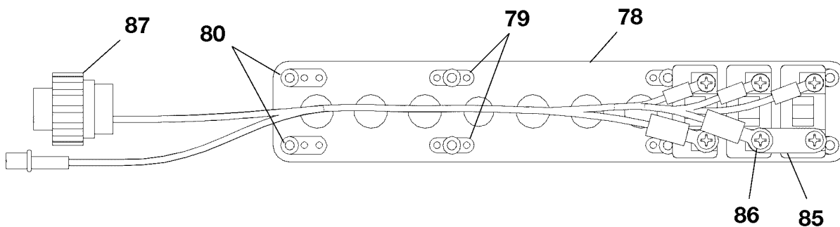
VIEW B-B
