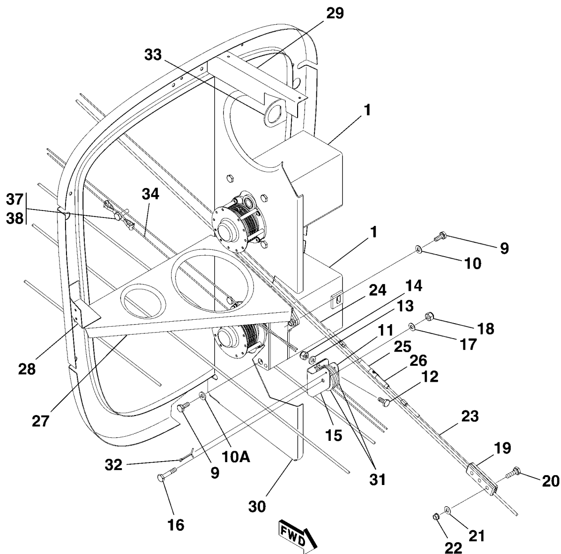
GFC-700 PITCH AND TRIM SERVO FIGURE 03 (SHEET 1)
