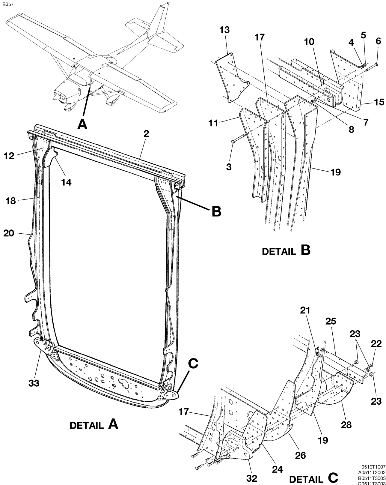
FORWARD DOORPOST BULKHEAD ASSEMBLY FIGURE 01 (SHEET 1)
