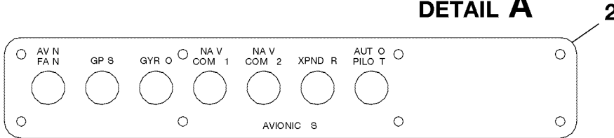
DETAIL A
