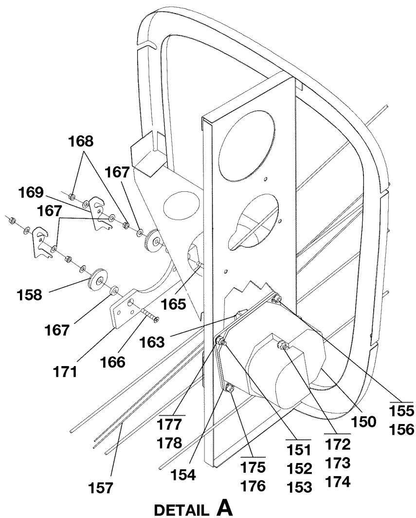
AUTOPILOT INSTALLATION KAP AND KC-140 FIGURE 01 (SHEET 3)
