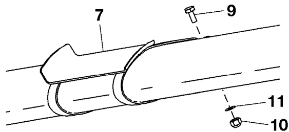
DETAIL B
