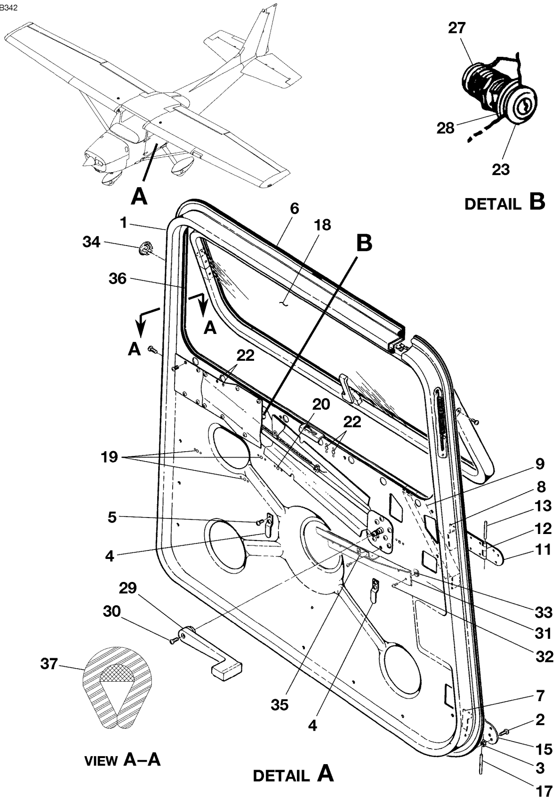
CABIN DOOR INSTALLATION - LH FIGURE 01 (SHEET 1)
