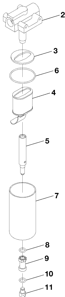
DETAIL A
