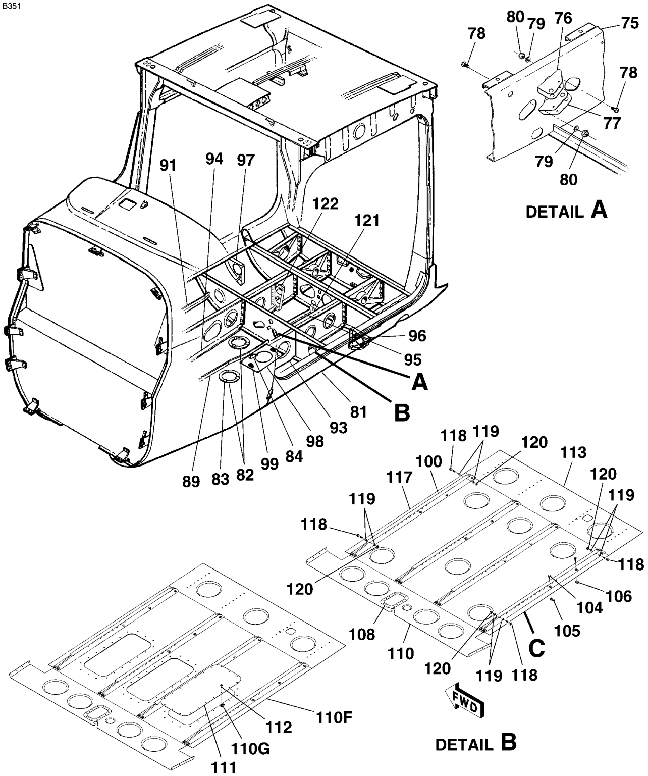
DETAIL C AIRPLANES 172S11621 AND ON FRONT AND CENTER SECTION ASSEMBLY-FUSELAGE FIGURE 01 (SHEET 2)
