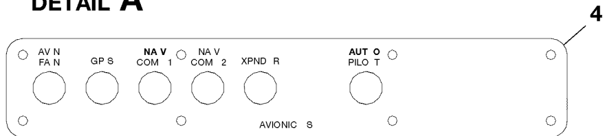
DETAIL A
