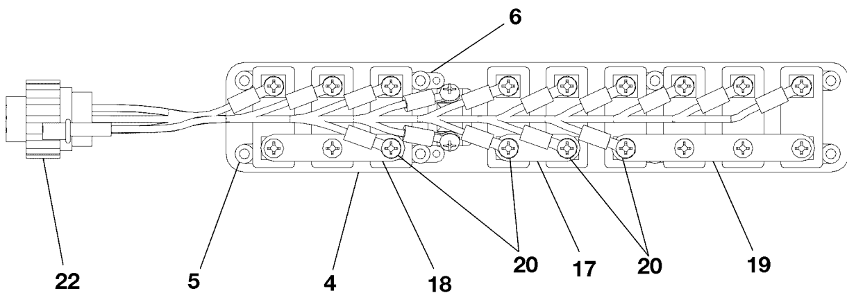
DETAIL B-B
