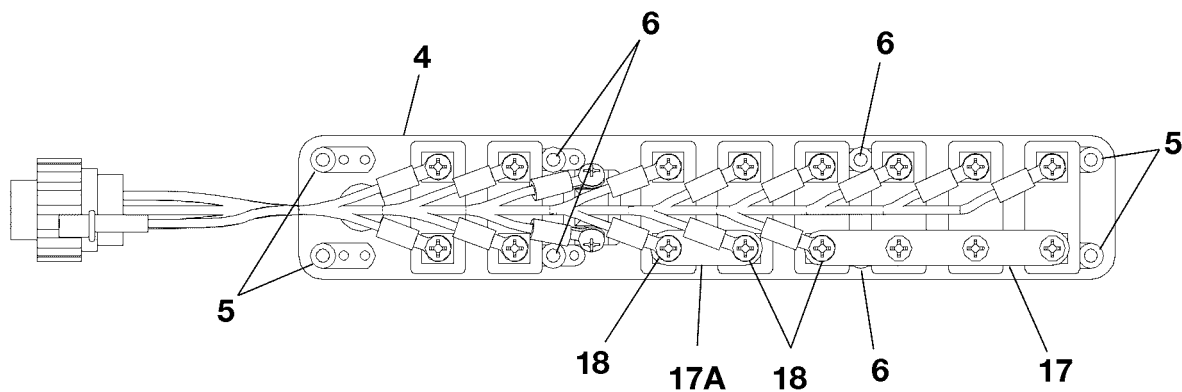
VIEW B-B
