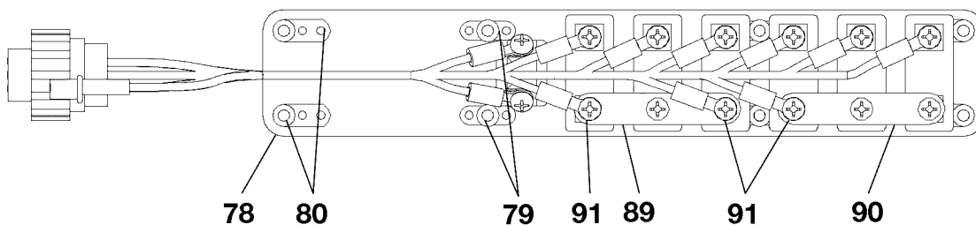
VIEW B-B
