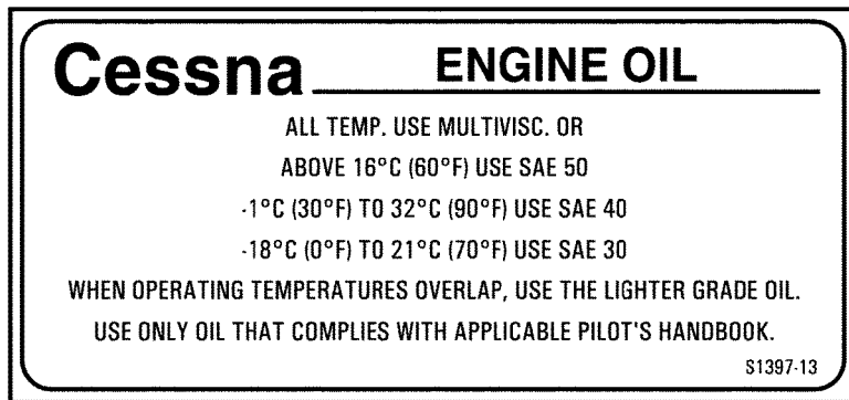
1 DETAIL A
