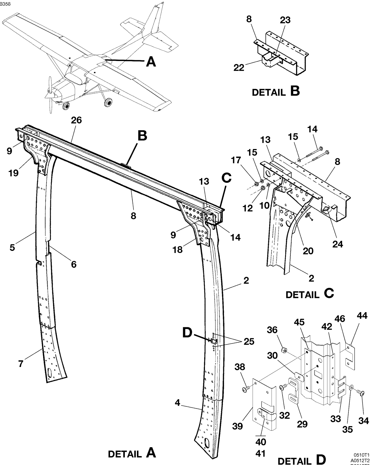
REAR DOORPOST BULKHEAD ASSEMBLY FIGURE 02 (SHEET 1)
