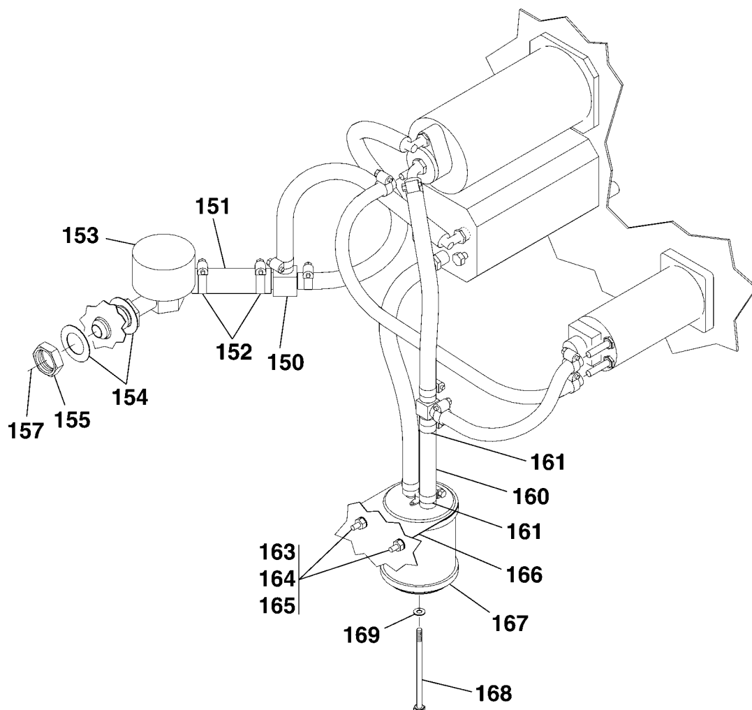
DETAIL A
