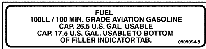
2 DETAIL B
