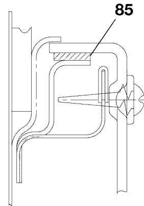
VIEW B-B
