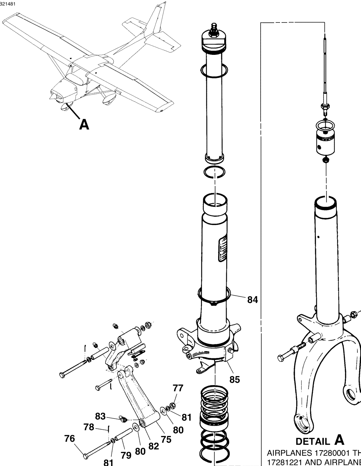
NOSE GEAR SHOCK STRUT ASSEMBLY FIGURE 01 (SHEET 2)
