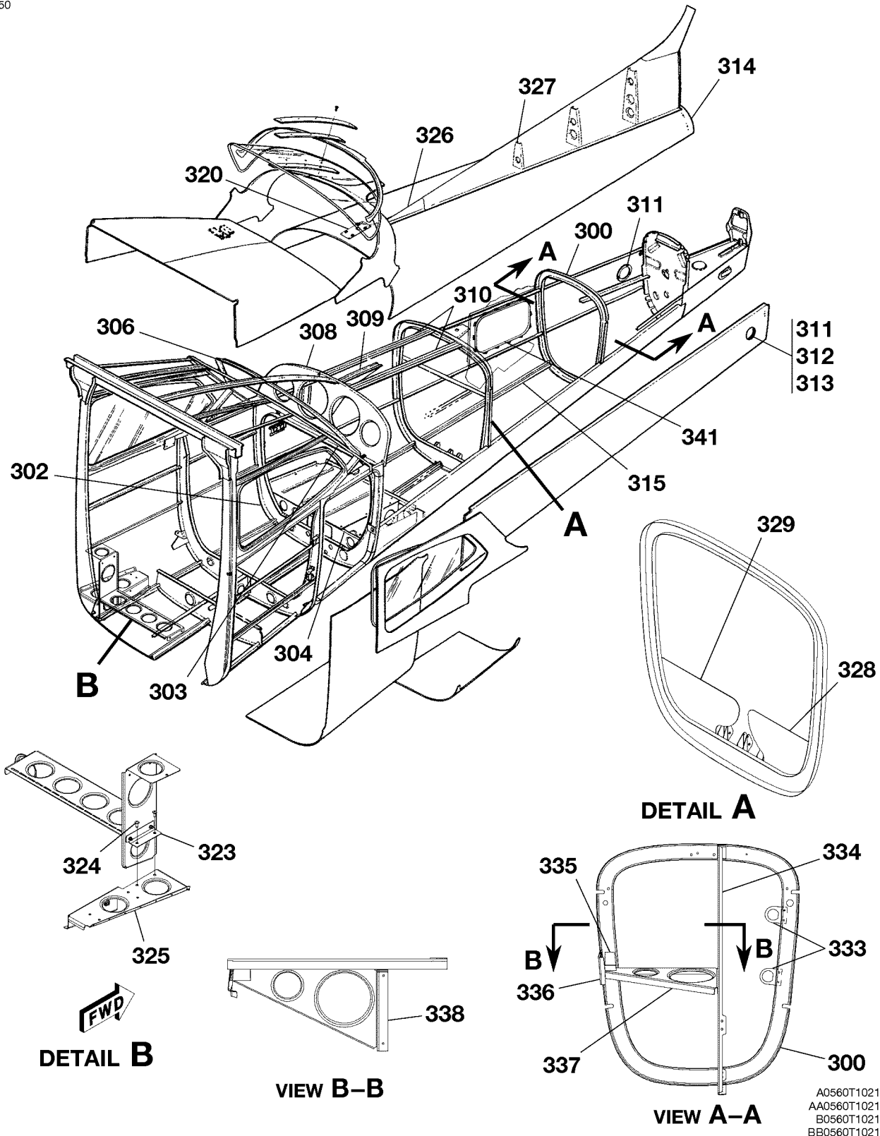
FUSELAGE AFT SECTION ASSEMBLY FIGURE 01 (SHEET 5)
