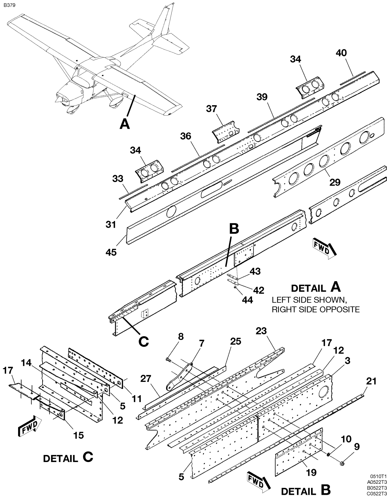
SPAR ASSEMBLIES - WING FIGURE 01 (SHEET 1)
