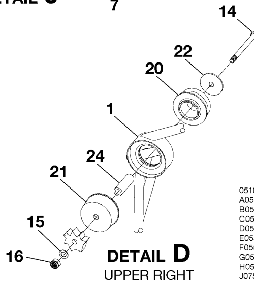
ENGINE MOUNT INSTALLATION FIGURE 01 (SHEET 1)
