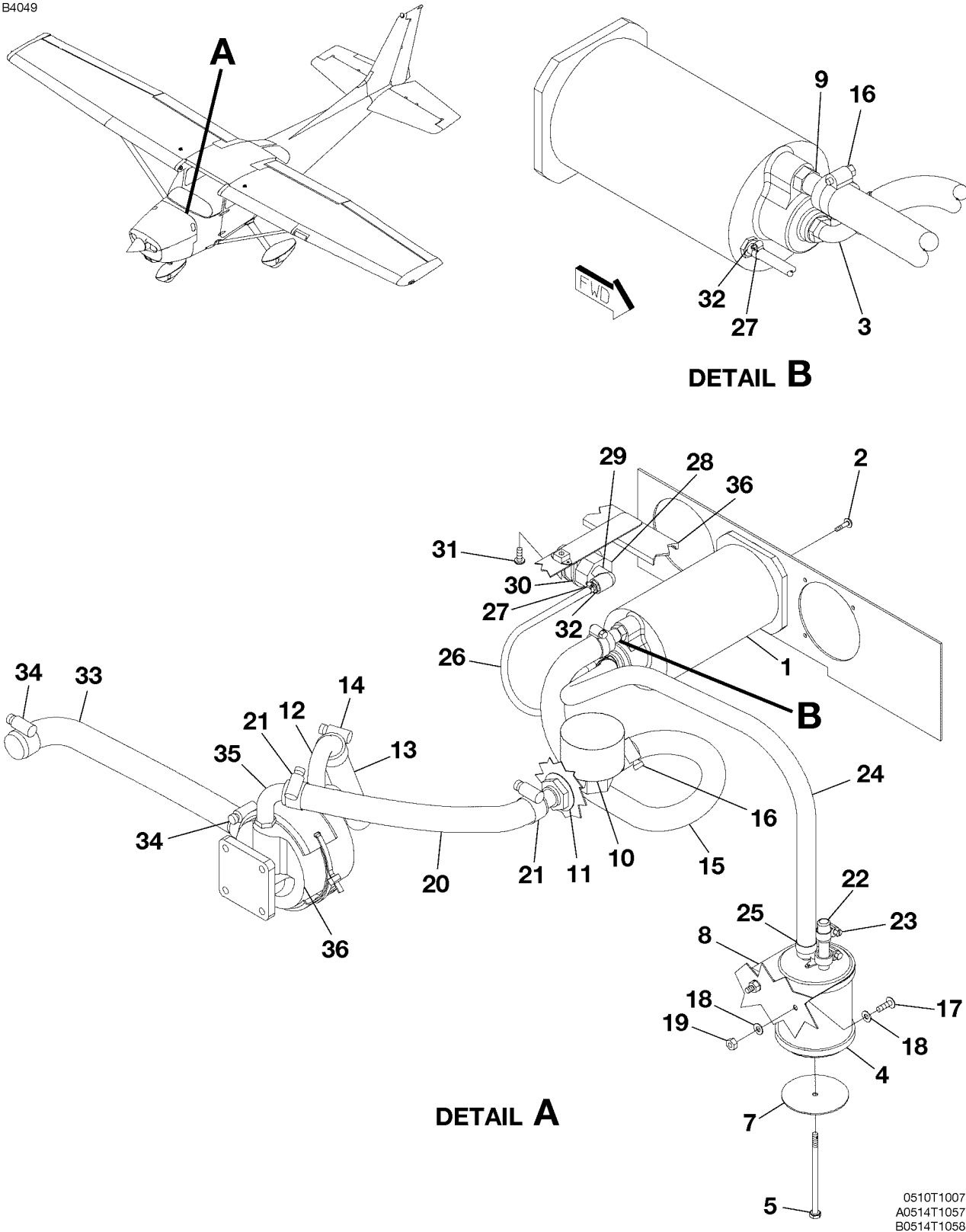
GYRO AND VACUUM INSTALLATION - NAV III FIGURE 07 (SHEET 1)
