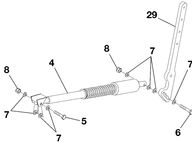
DETAIL A
