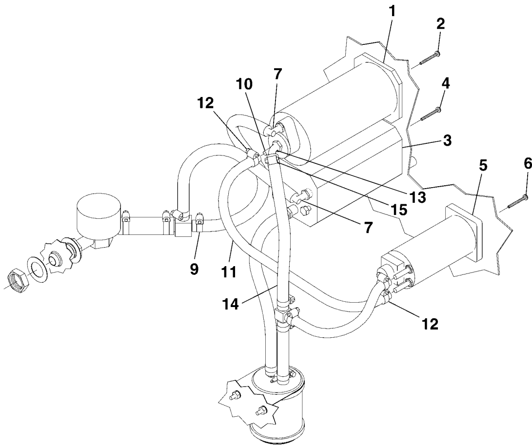
DETAIL A
