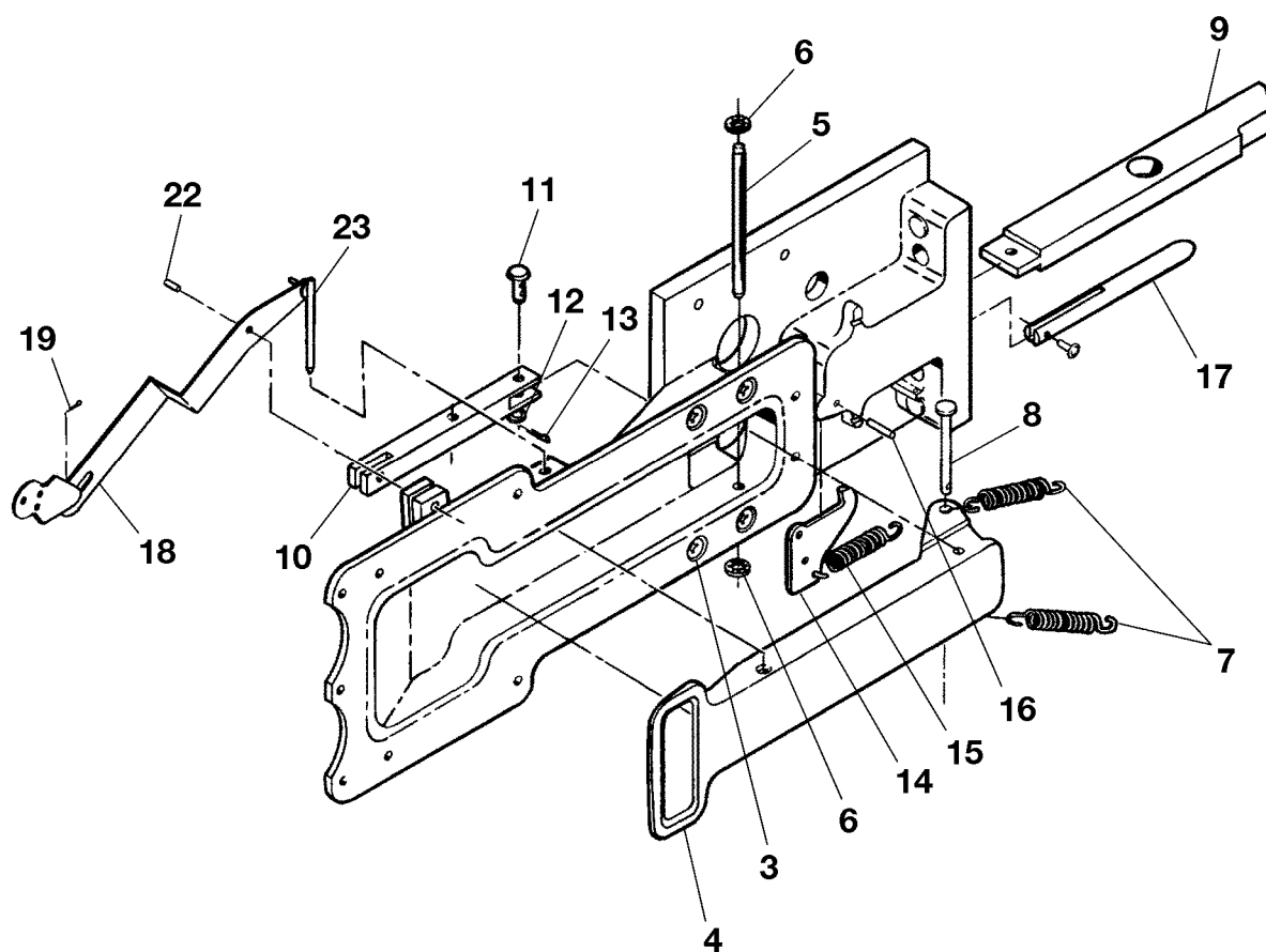
DETAIL A
