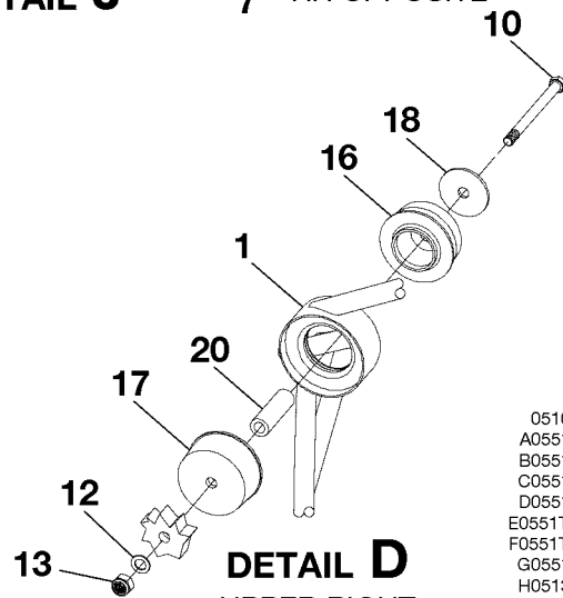
ENGINE MOUNT INSTALLATION FIGURE 03 (SHEET 1)
