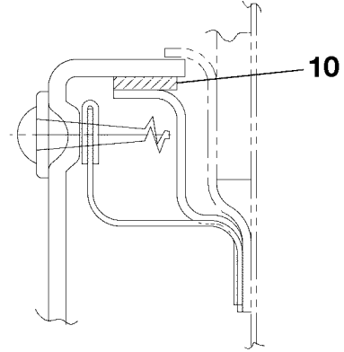
VIEW B-B
