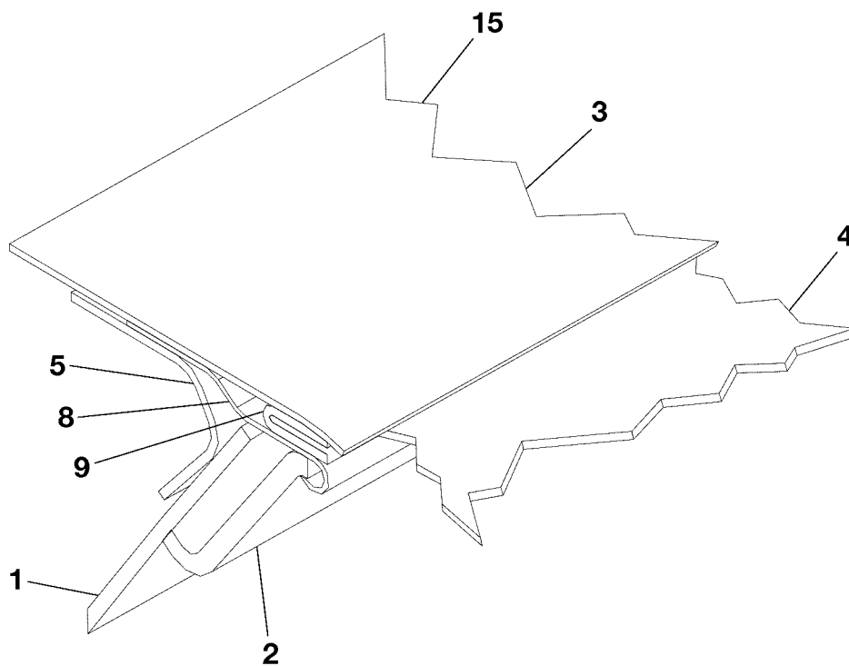
DETAIL A
