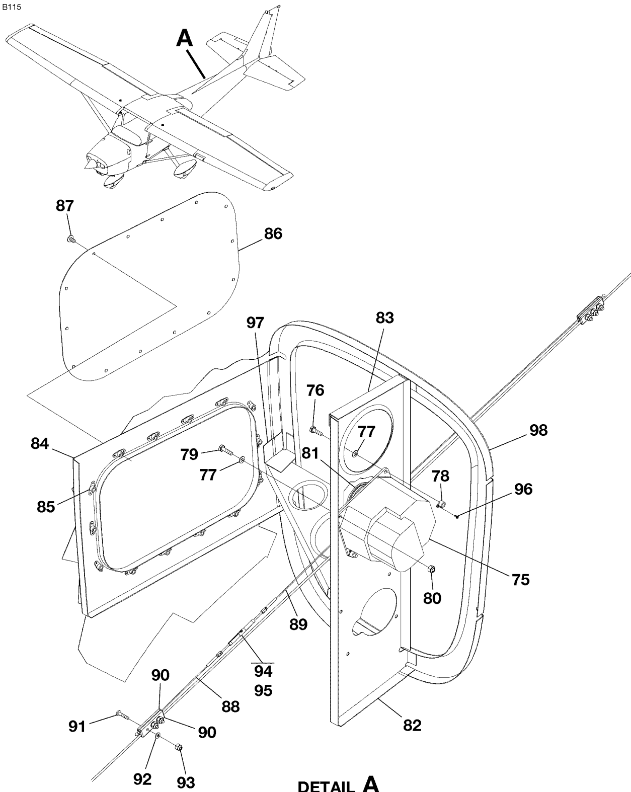
AUTOPILOT INSTALLATION KAP AND KC-140 FIGURE 01 (SHEET 2)
