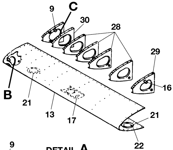
DETAIL A
