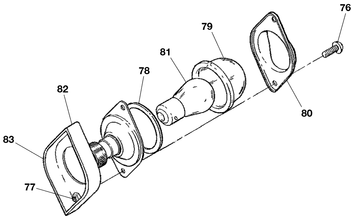
DETAIL A
