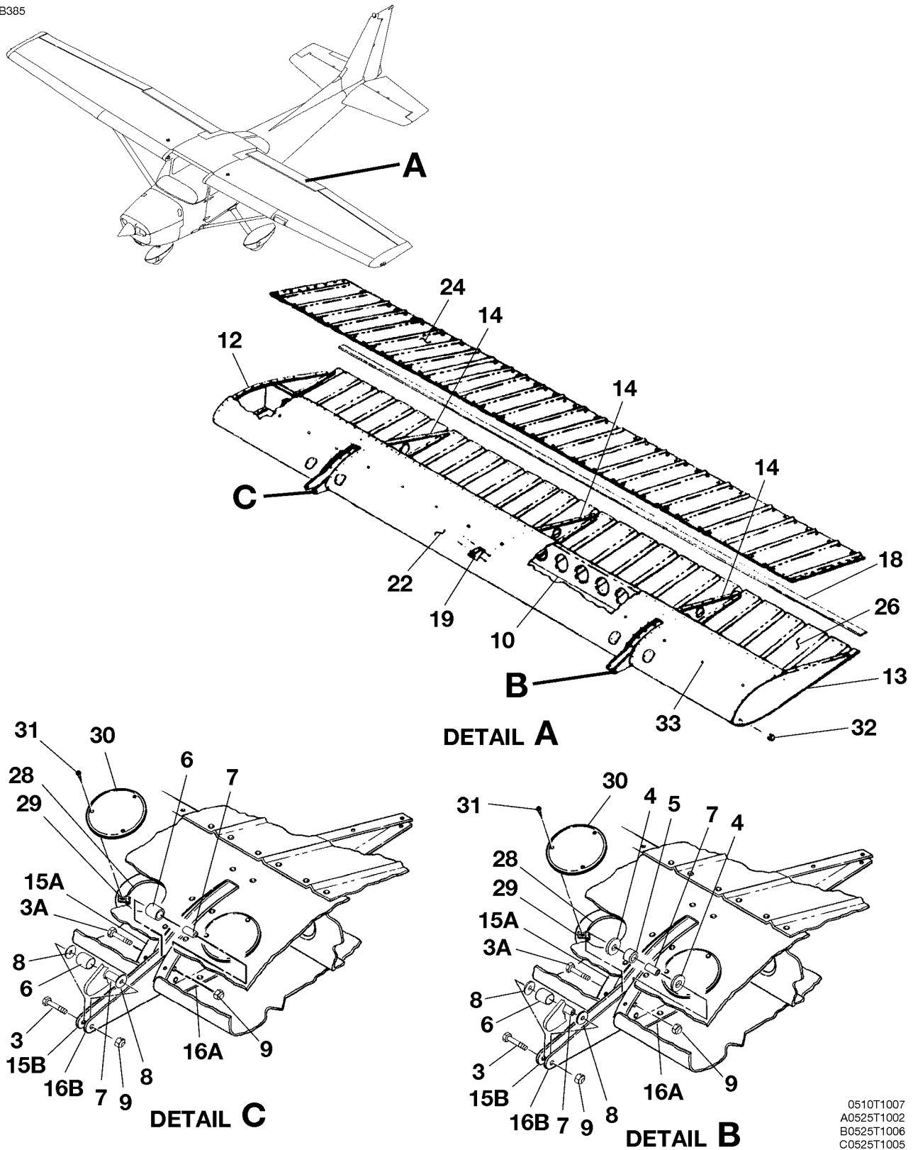
FLAP INSTALLATION FIGURE 01 (SHEET 1)
