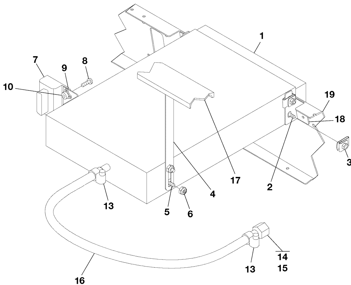
DETAIL A
