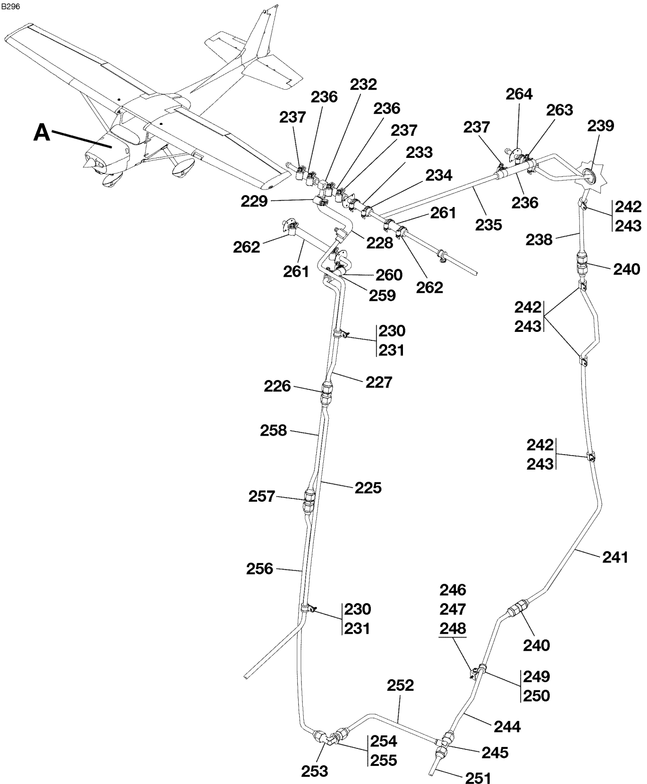
FUEL SYSTEM FIGURE 01 (SHEET 4)
