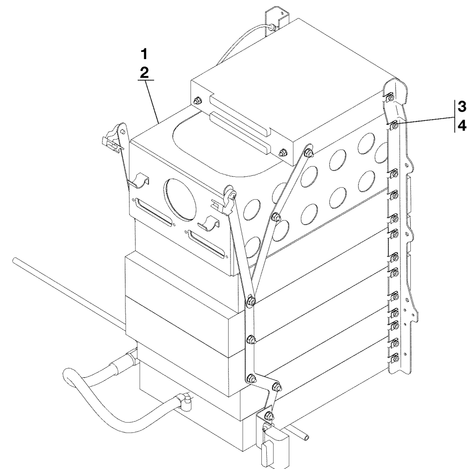
DETAIL A
