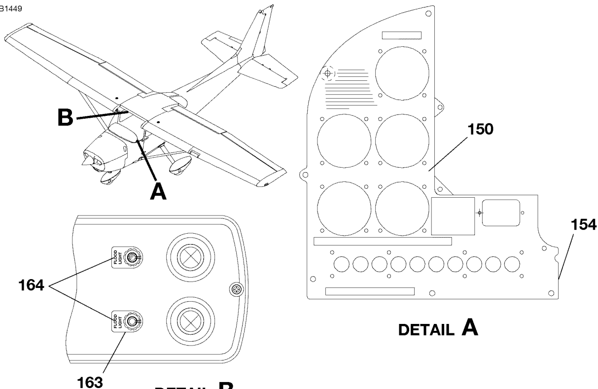
DETAIL B NAV III OVERHEAD CONSOLE SILKSCREEN
