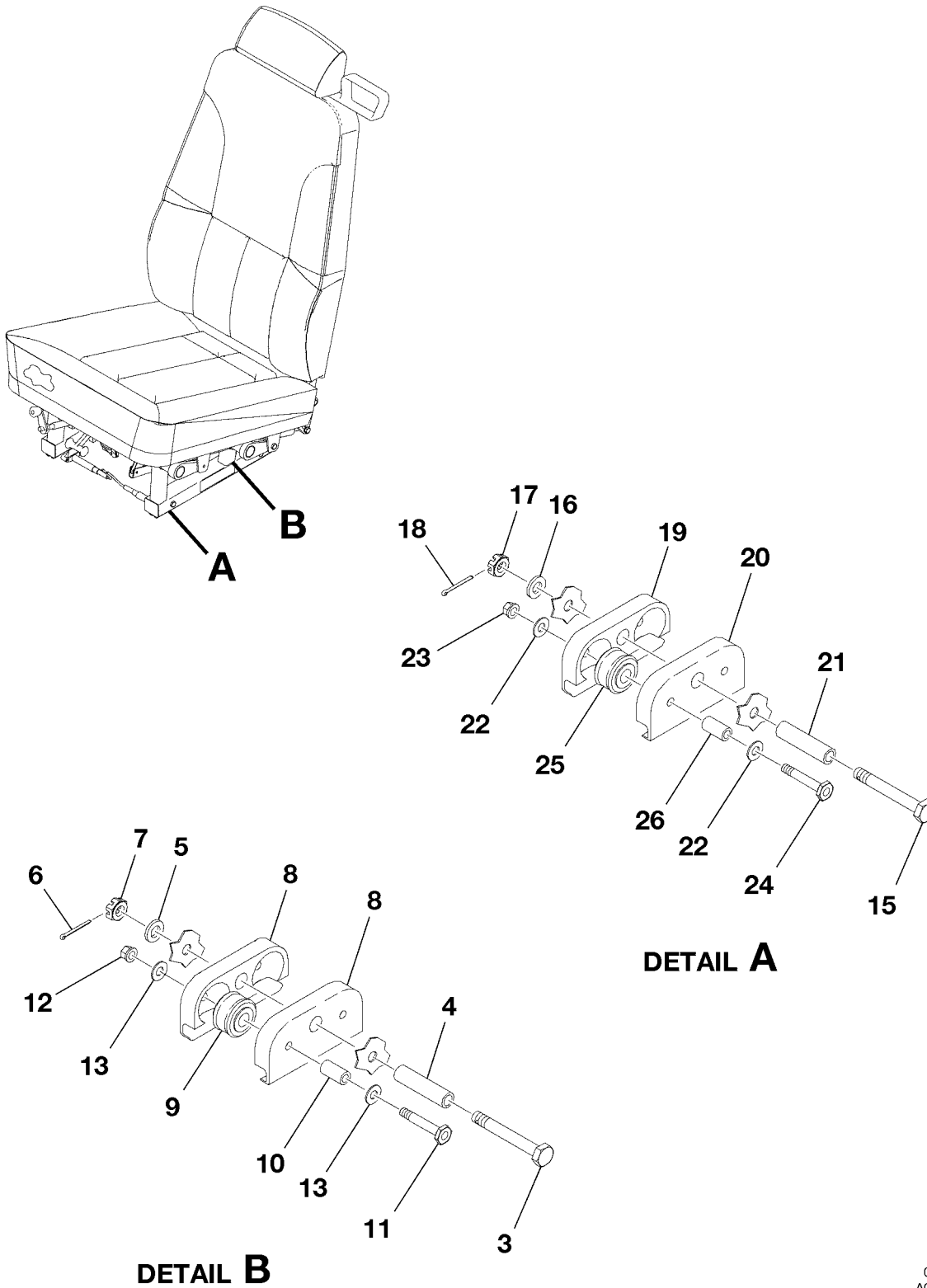
SEAT FOOT ASSY-PILOT AND COPILOT FIGURE 04 (SHEET 1)
