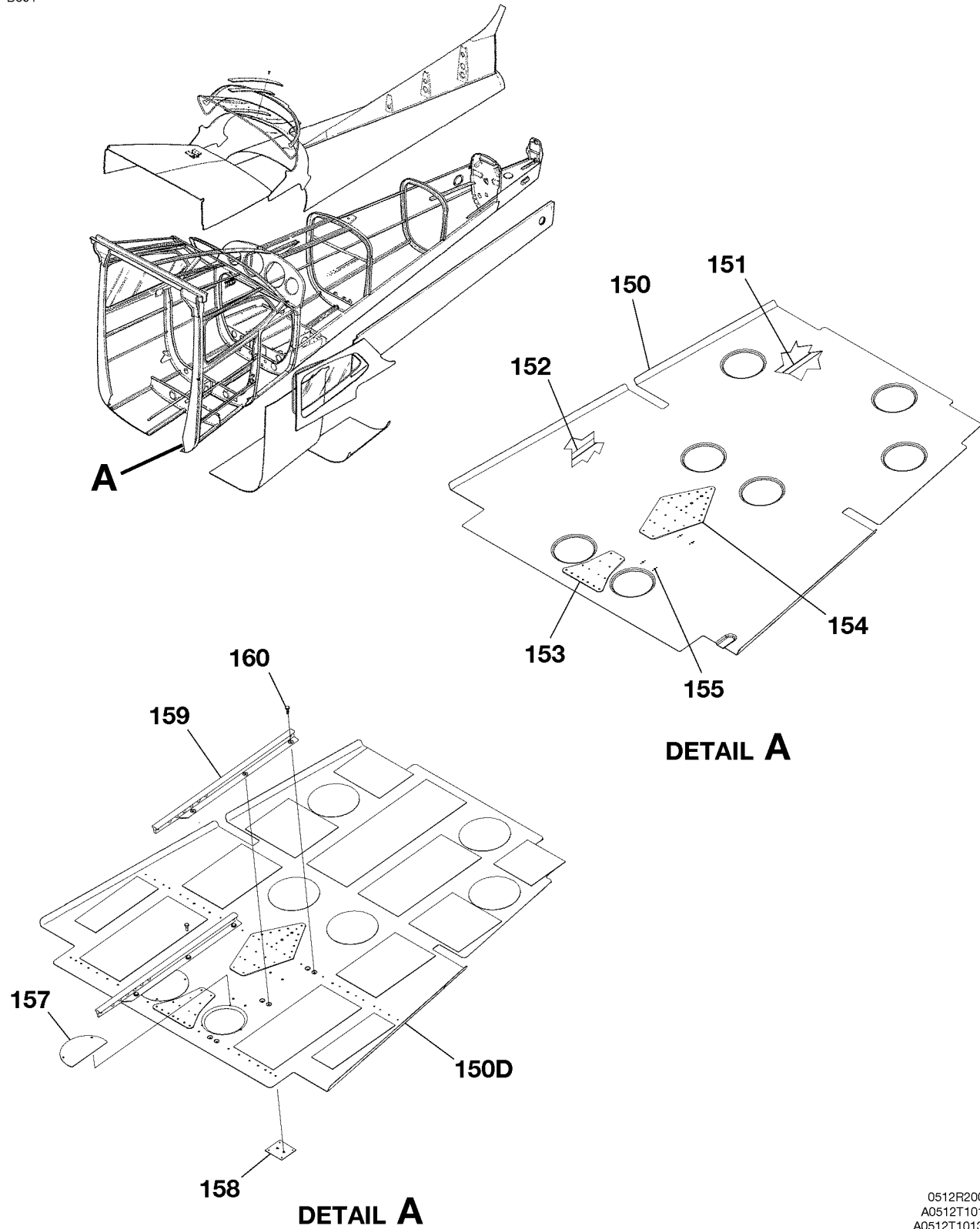
FUSELAGE AFT SECTION ASSEMBLY FIGURE 01 (SHEET 3)
