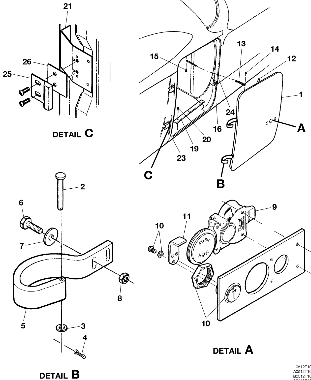
BAGGAGE DOOR INSTALLATION FIGURE 01 (SHEET 1)
