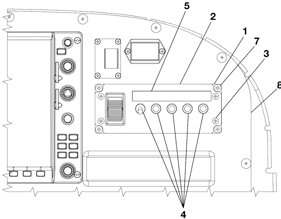
DETAIL B
