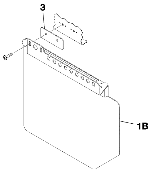
DETAIL A
