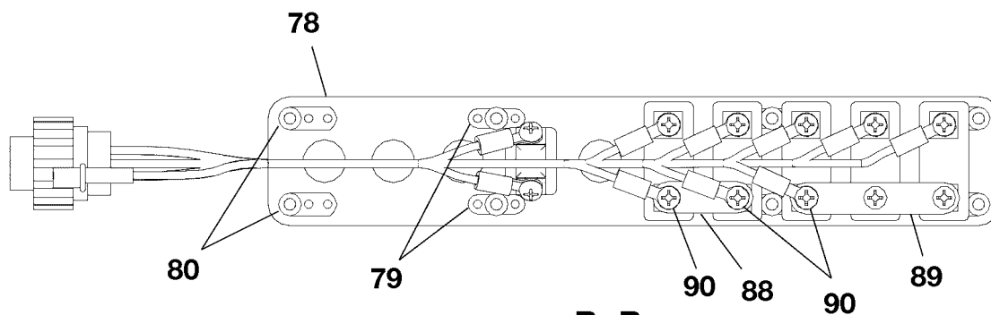
VIEW B-B
