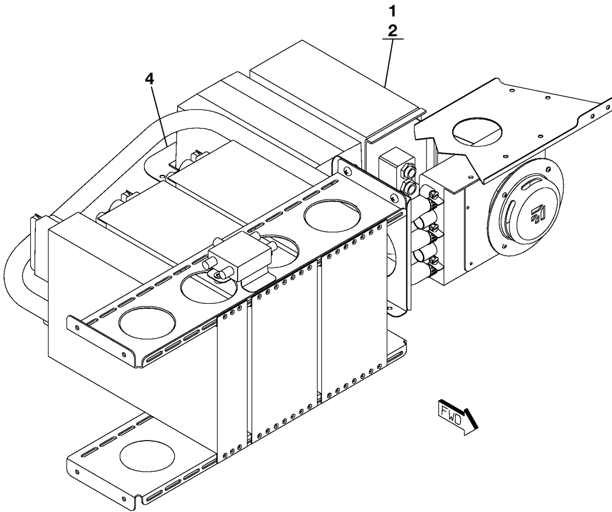
DETAIL A
