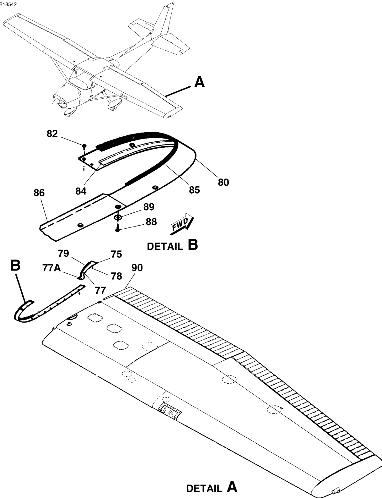
WING INSTALLATION FIGURE 01 (SHEET 2)
