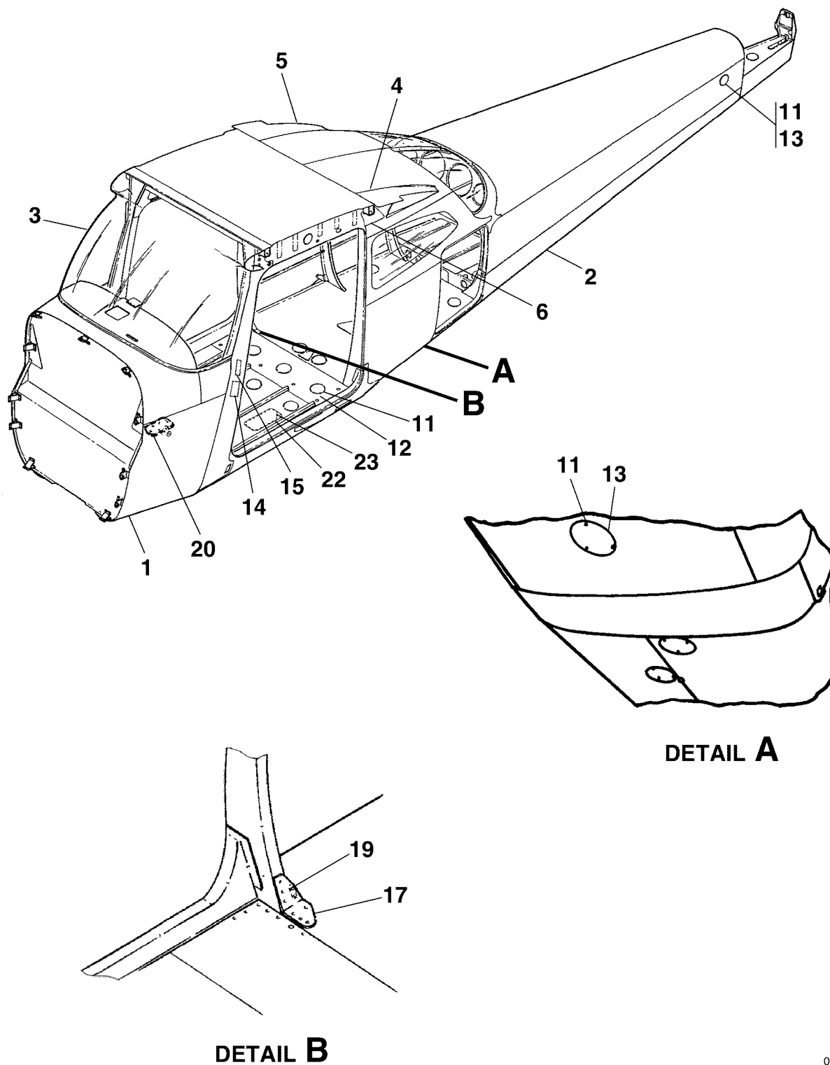
FUSELAGE ASSEMBLY FIGURE 01 (SHEET 1)
