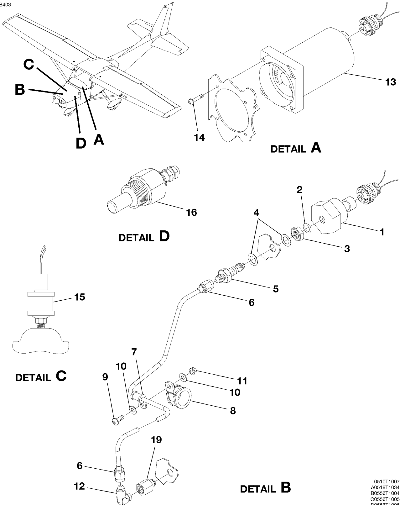
OIL INDICATING SYSTEM FIGURE 01 (SHEET 1)
