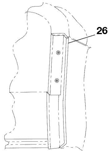
VIEW B-B
