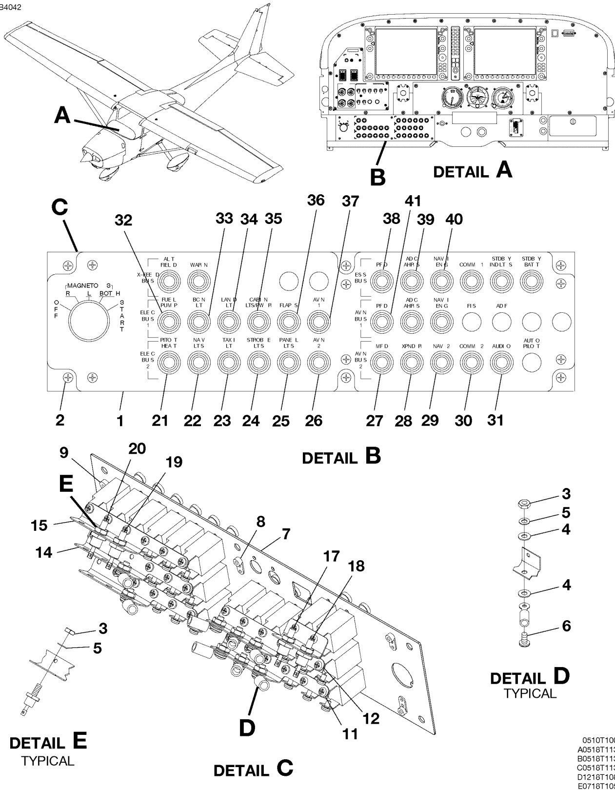
CIRCUIT BREAKER PANEL ASSEMBLY-NAV III FIGURE 01B (SHEET 1)
