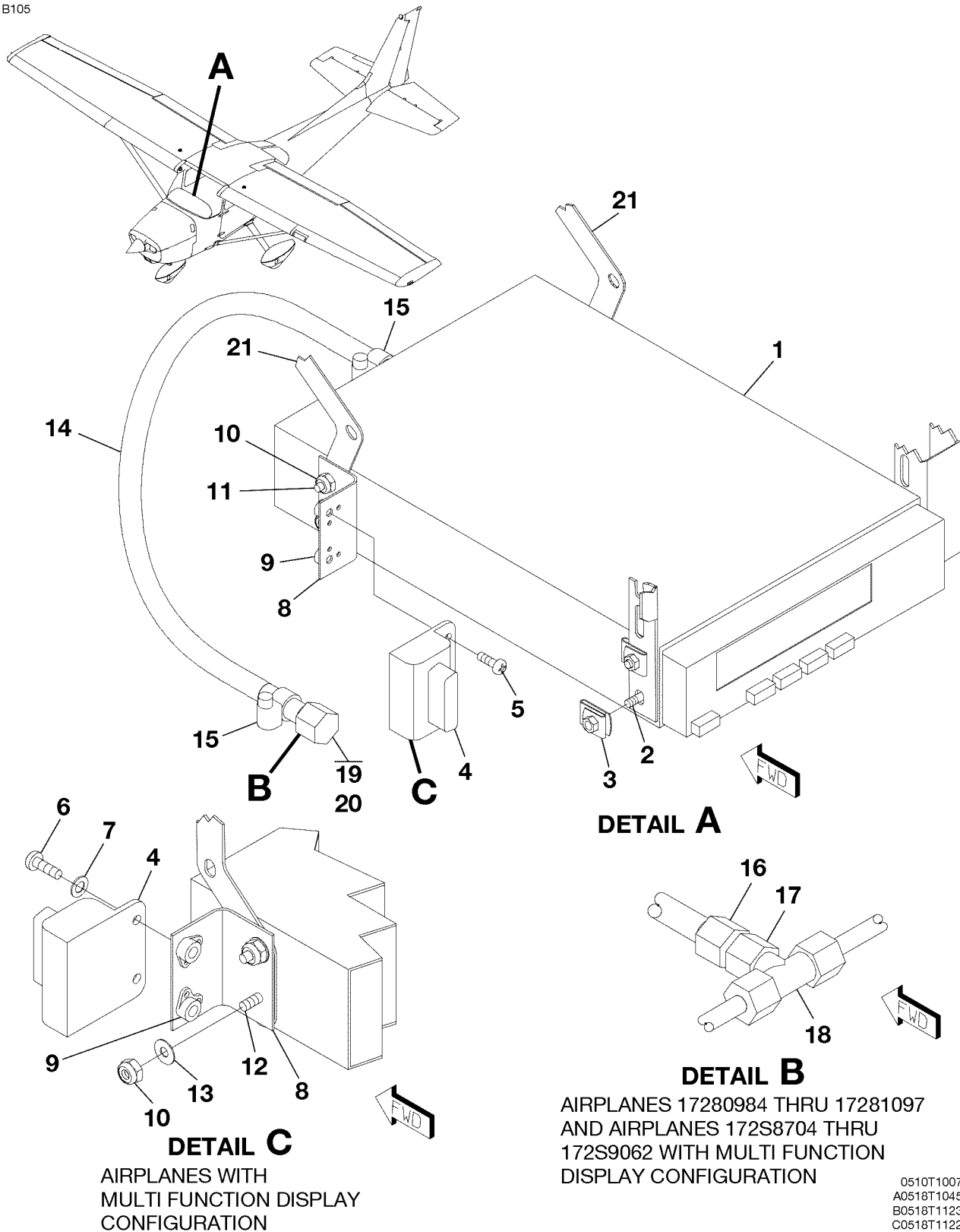
AUTOPILOT INSTALLATION KAP AND KC-140 FIGURE 01 (SHEET 1)
