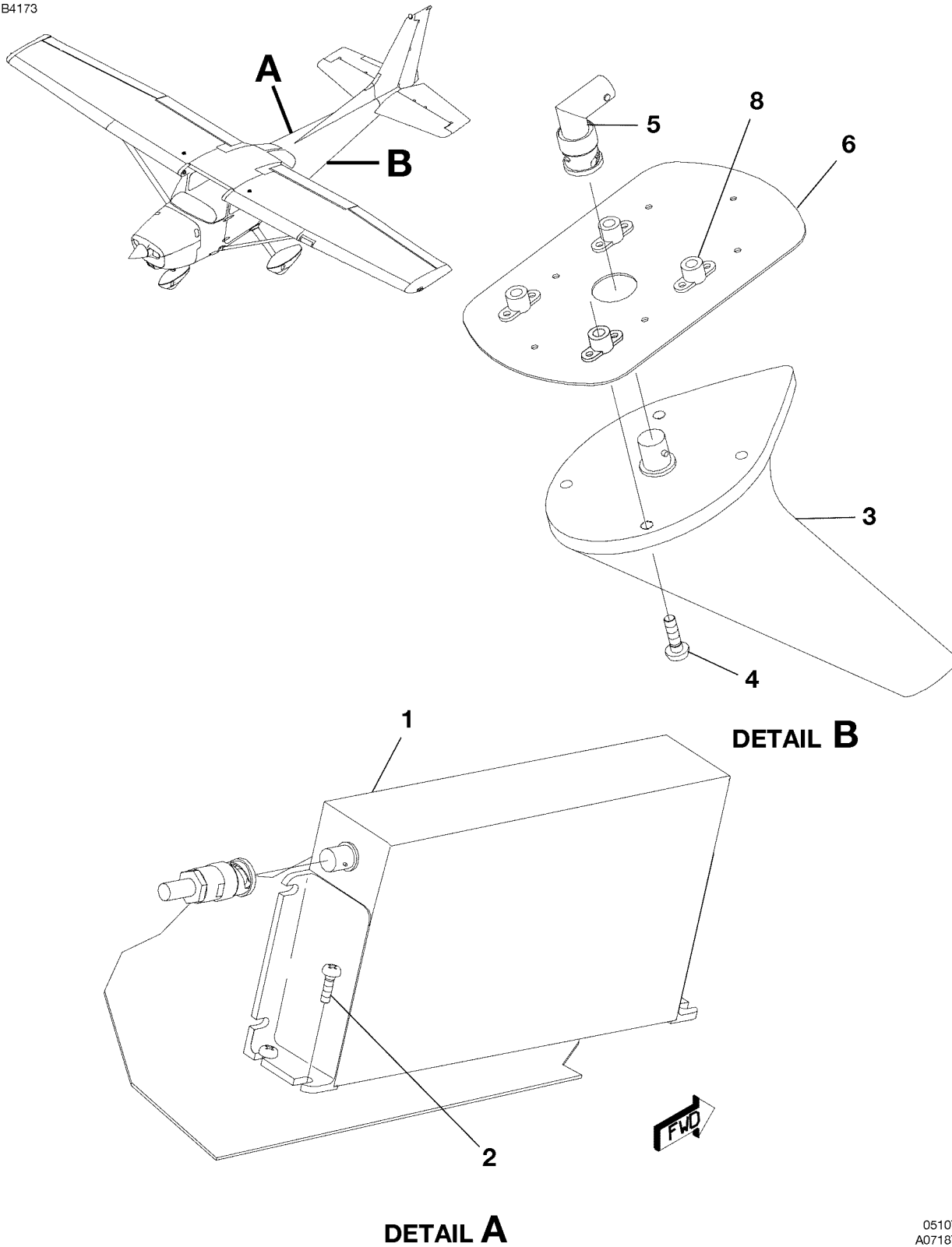
FLIGHT INFORMATION SERVICES (FIS) RECEIVER AND ANTENNA INSTALLATION FIGURE 04 (SHEET 1)
