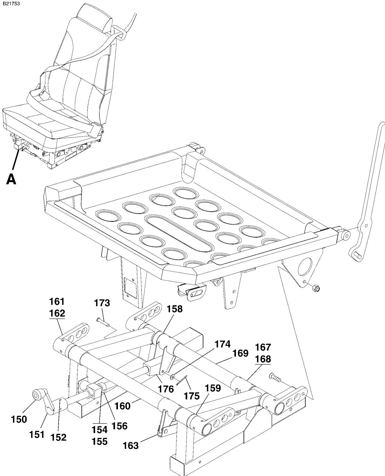
SEAT ASSEMBLY - PILOT AND COPILOT FIGURE 03 (SHEET 3)
