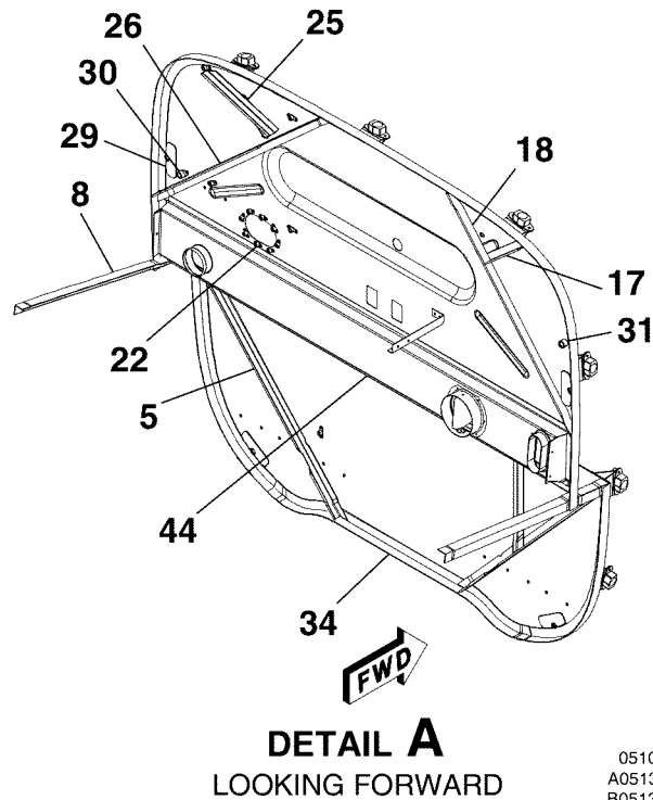
FIREWALL ASSEMBLY FIGURE 01A (SHEET 1)
