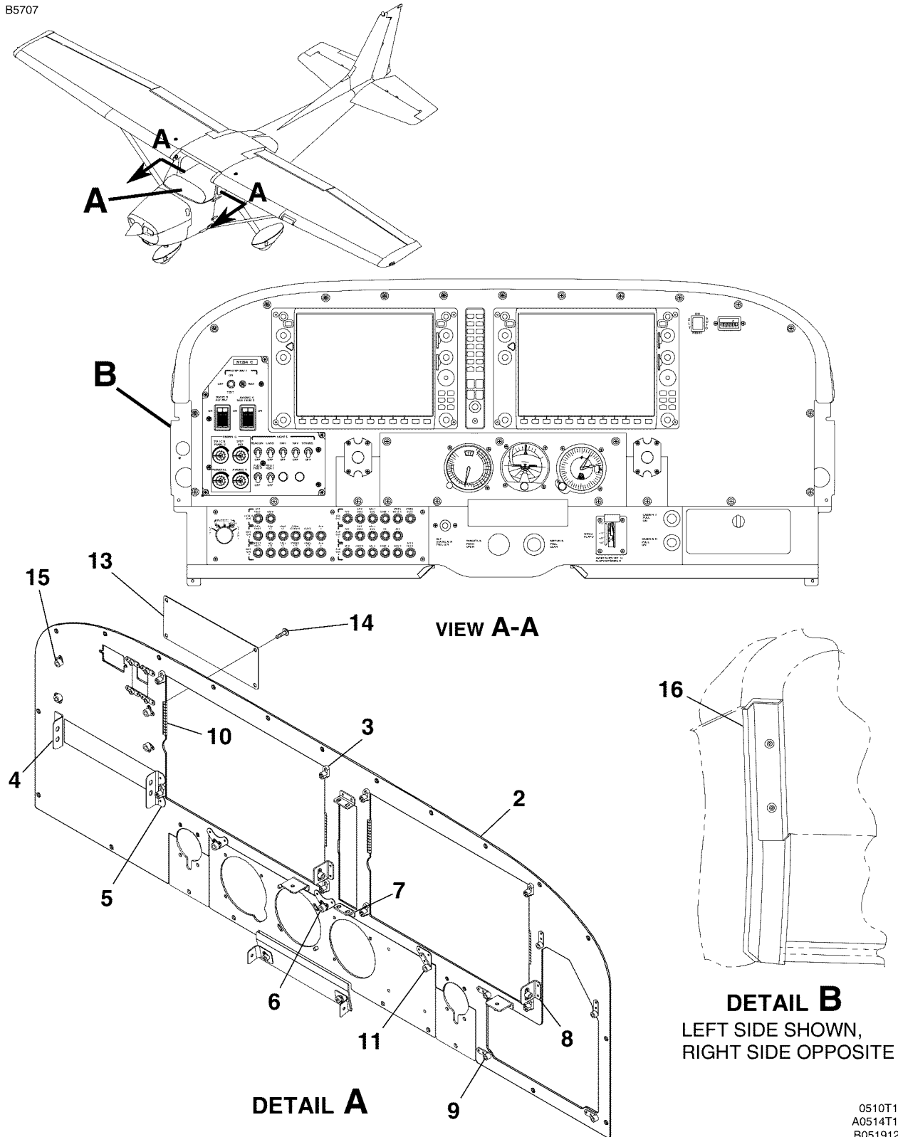
INSTRUMENT PANEL ASSEMBLY-NAV III WITH ADF, ELT, ELT/ADF FIGURE 01B (SHEET 1)
