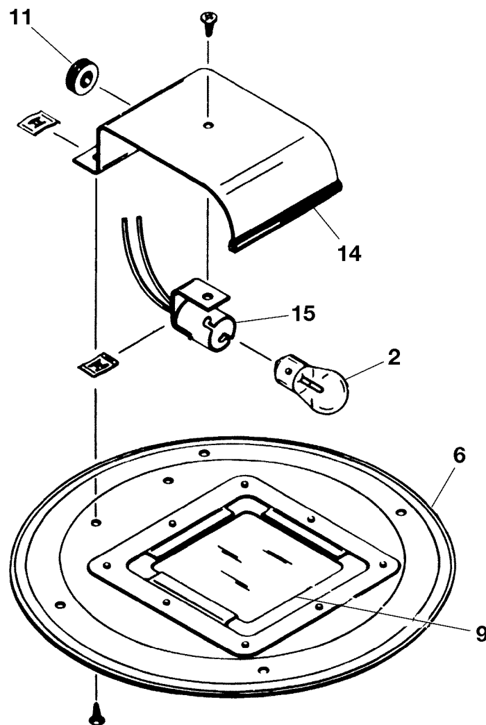
DETAIL A
