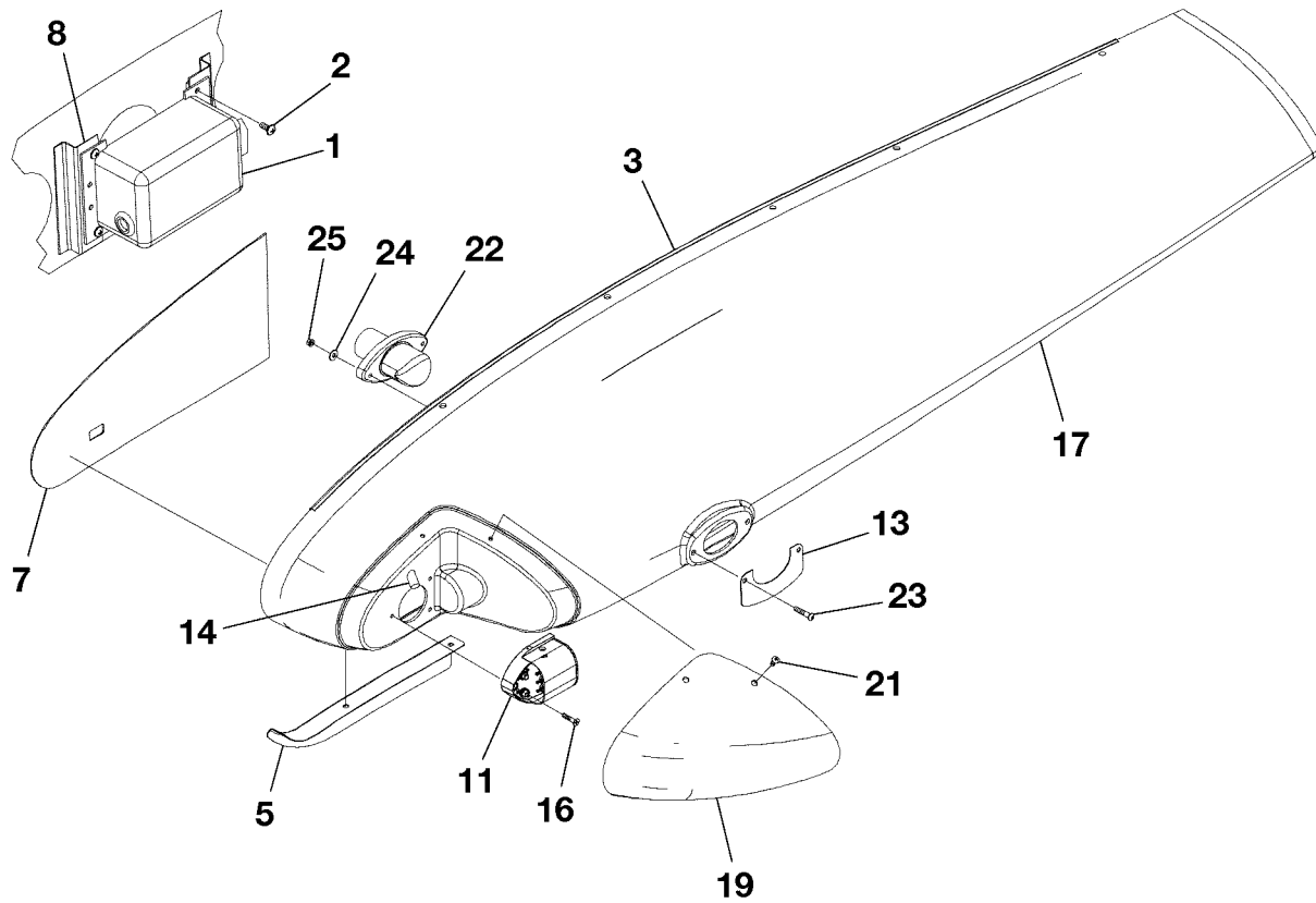
DETAIL A
