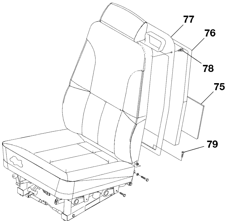
SEAT INSTALLATION - PILOT AND COPILOT FIGURE 01 (SHEET 2)
