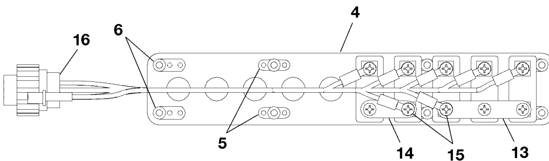
VIEW B-B
