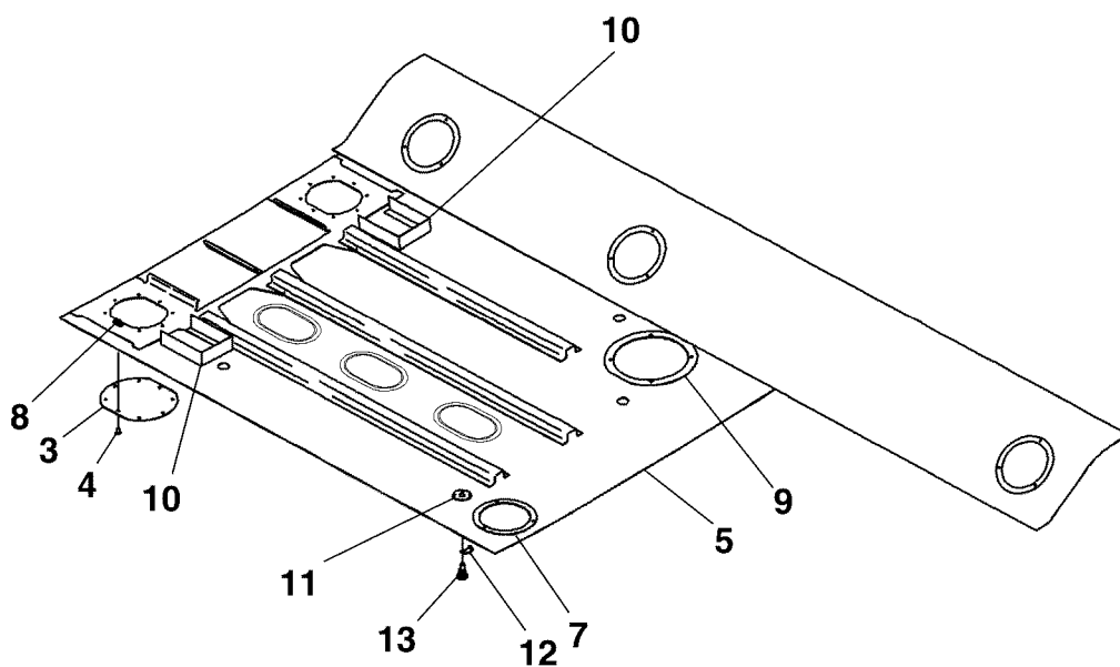
DETAIL A
