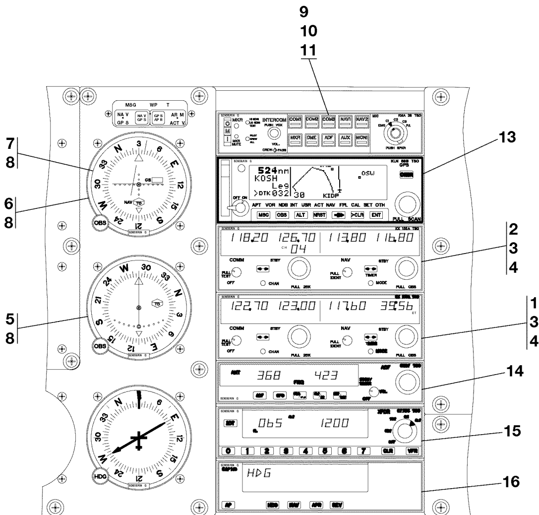
DETAIL B
