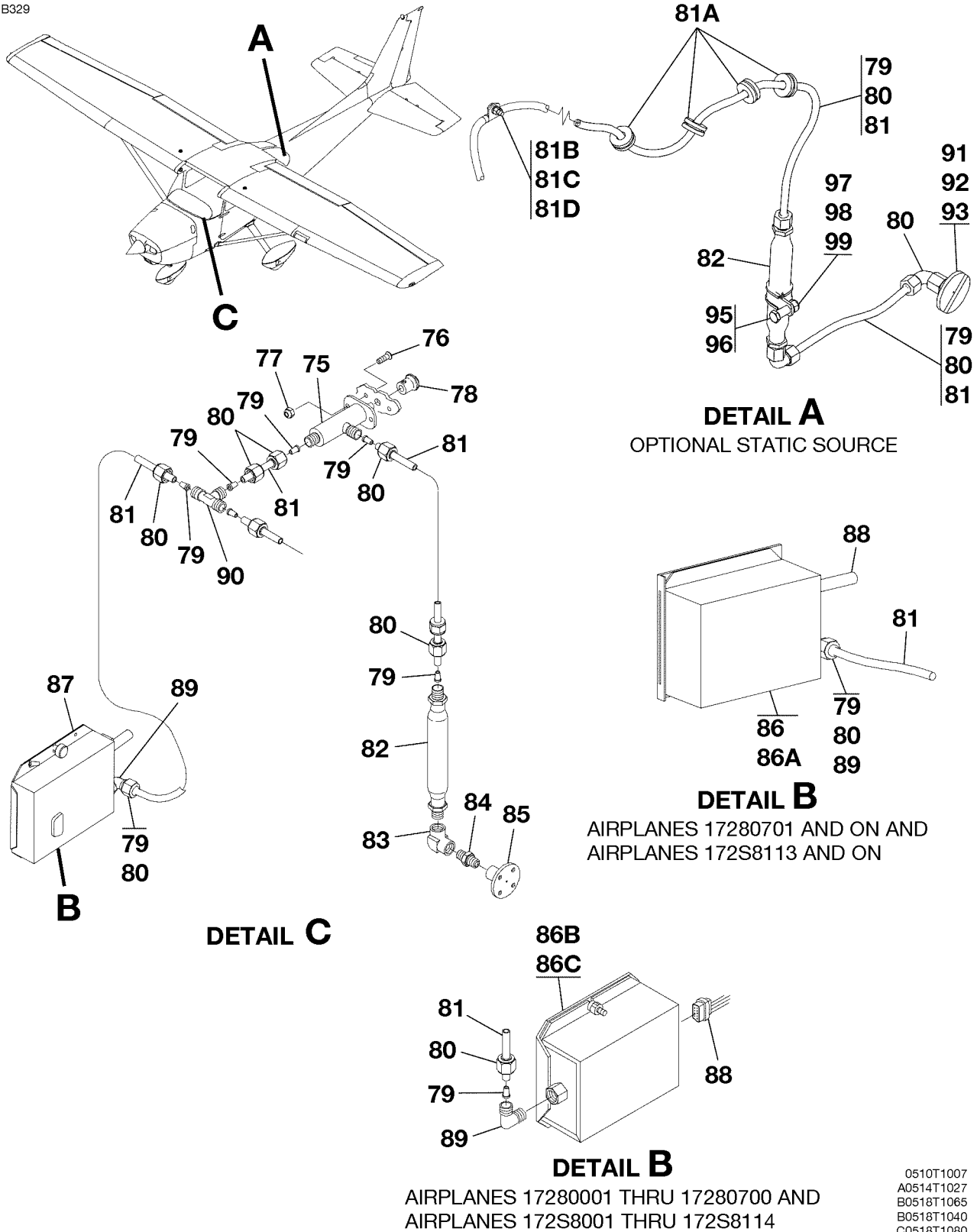
PITOT AND STATIC SYSTEM FIGURE 01 (SHEET 2)
