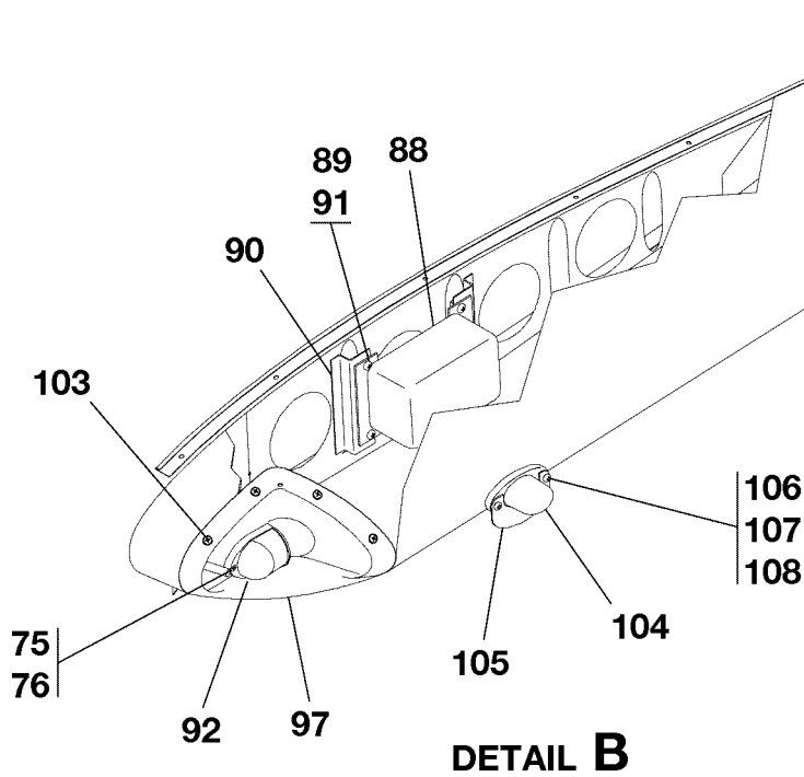
LIGHTING - NAVIGATION WING AND TAIL FIGURE 02 (SHEET 2)
