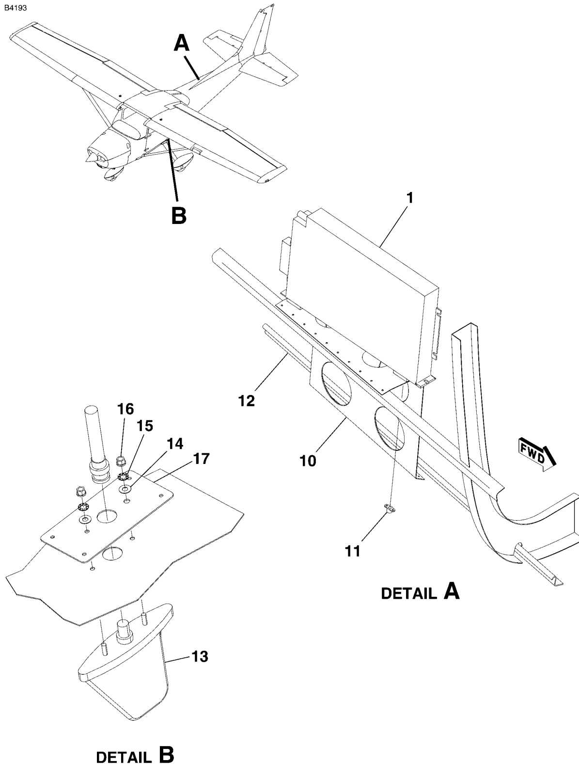
DISTANCE MEASURING EQUIPMENT (DME) INSTALLATION FIGURE 02 (SHEET 1)
