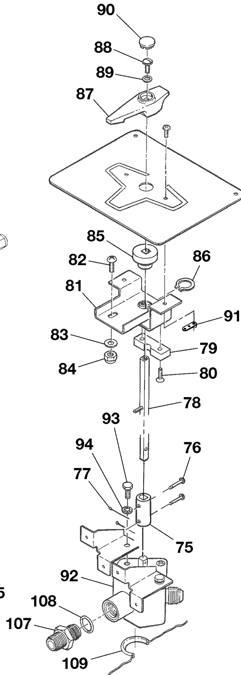
DETAIL A
